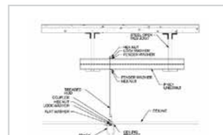
Hanging Ceiling
