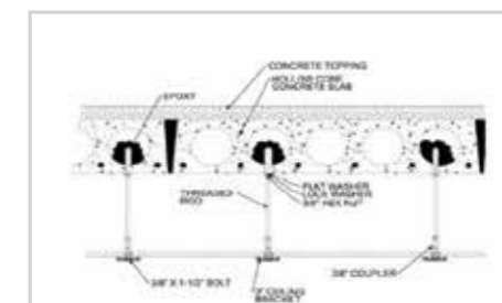
Hollow-Core Concrete
